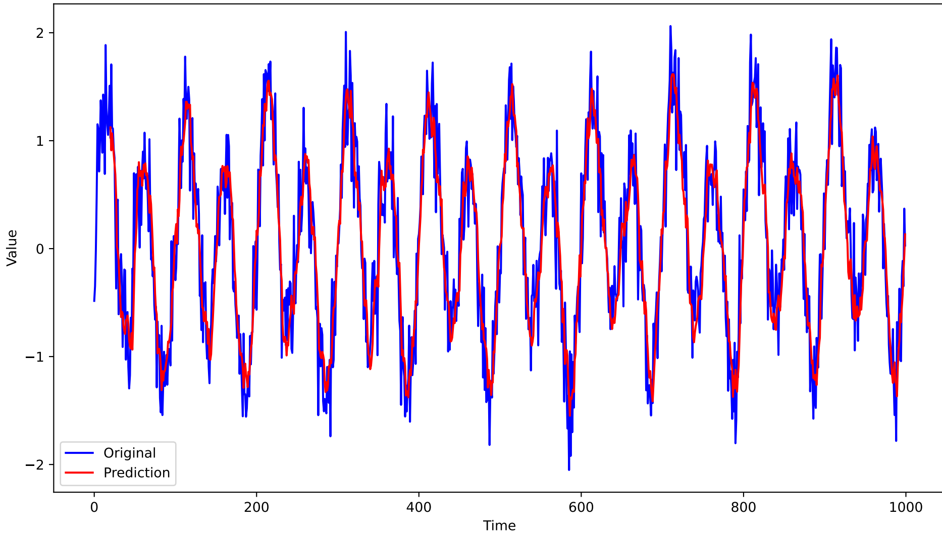
AR(20) LS one step prediction
